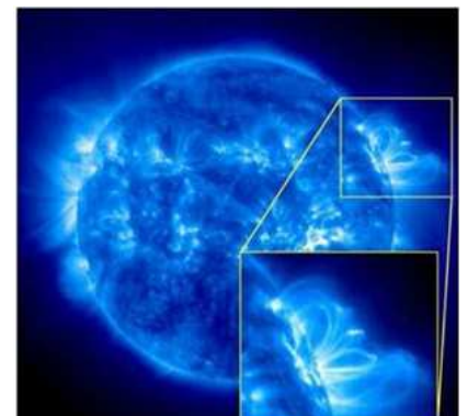
Figure 2 SOHO/EIT Image with a Coronal Loop Region on the outside of the Sun
