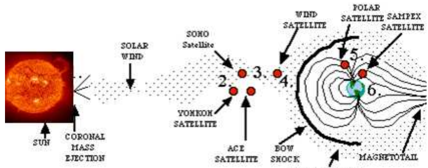
Figure 1 The interaction between the Sun and Earth along with the designated satellites [10]
