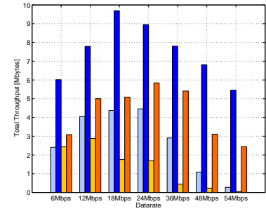
Figure 5: Total traffic delivered to an AP versus a parked vehicle per contact.
