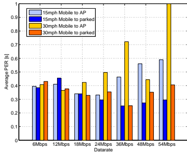
Figure 3: Average PER during a contact.
