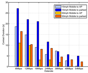
Figure 4: Link duration to an AP Vs a link between moving and parked vehicles.
