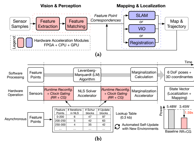
Figure 3: RoboAcc [2, 7, 19, 33, 34, 38] features (a) unified autonomy algorithm framework and (b) runtime-reconfigurable hardware accelerator for efficient and adaptive AMC.
