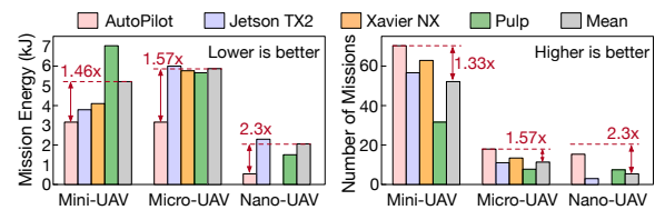
Figure 5: Skyline-AutoPilot quickly explores huge design space and consistently generates optimal AMC designs across scenarios.
