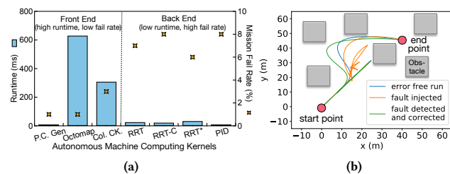
Figure 7: MAVFI-BERRY accurately evaluate end-to-end AMC resilience and significantly improve AMC resilience with low overhead.
