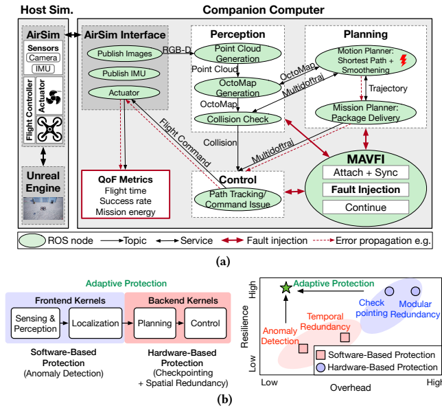
Figure 4: MAVFI-VPP-BERRY [11, 29, 30, 32, 35, 36] proposes (a) end-to-end resilience analysis framework and (b) adaptive protection with performance-efficiency optimization for resilient AMC.
