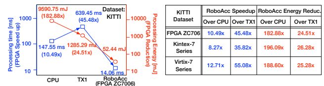
Figure 6: RoboAcc efficiently processes AMC kernels in real-time and is adaptive to dynamically changing environments.
